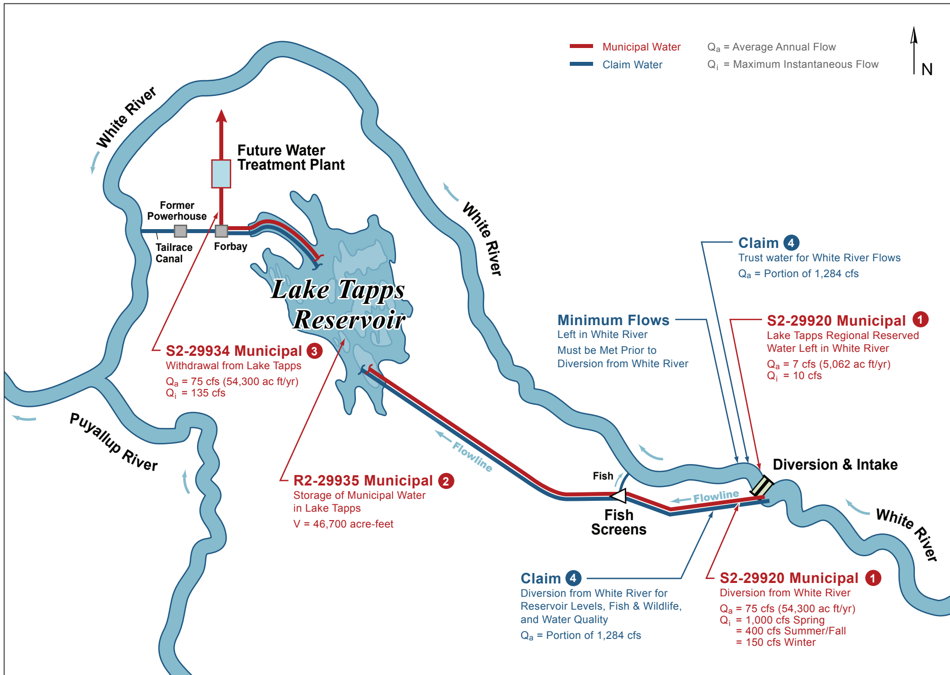
Figure FS-1. Schematic of the Water Right Applications and Change of Use Application
